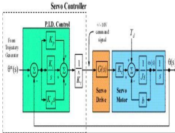
Figure 5: Using PID Controller to Control the Position of DC Servo Motor
