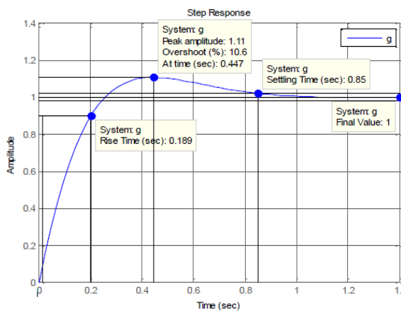
Figure 6: Step Response for PD Controller
